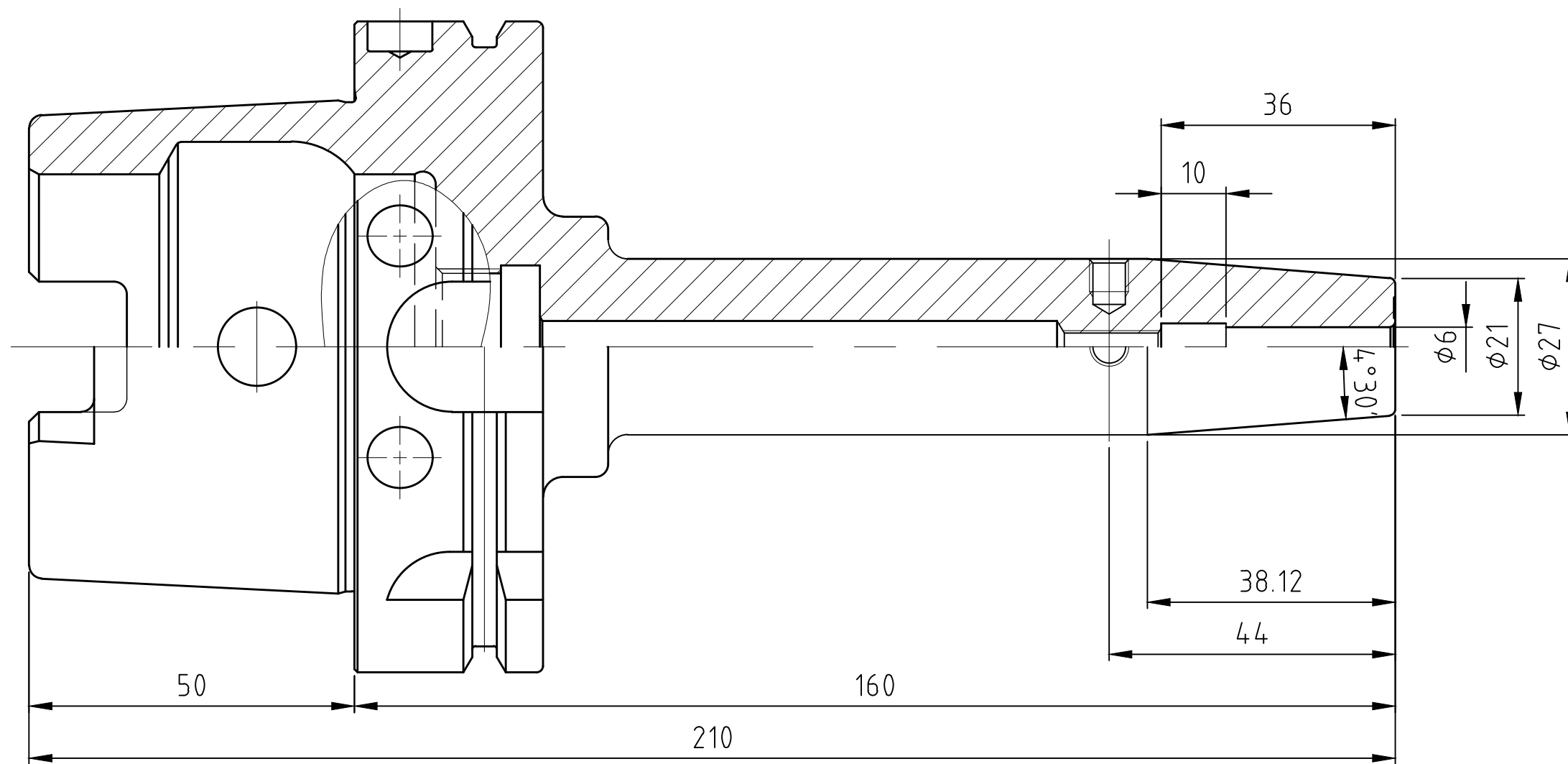
SECTION A'-A
