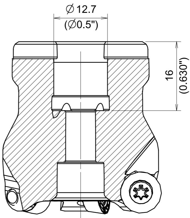
SECTION E-E
