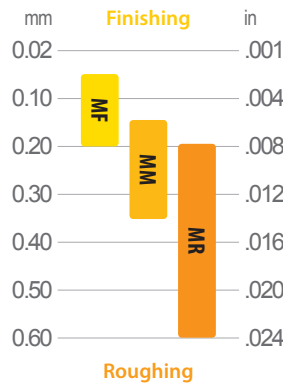
Feed Rate (Fn)
